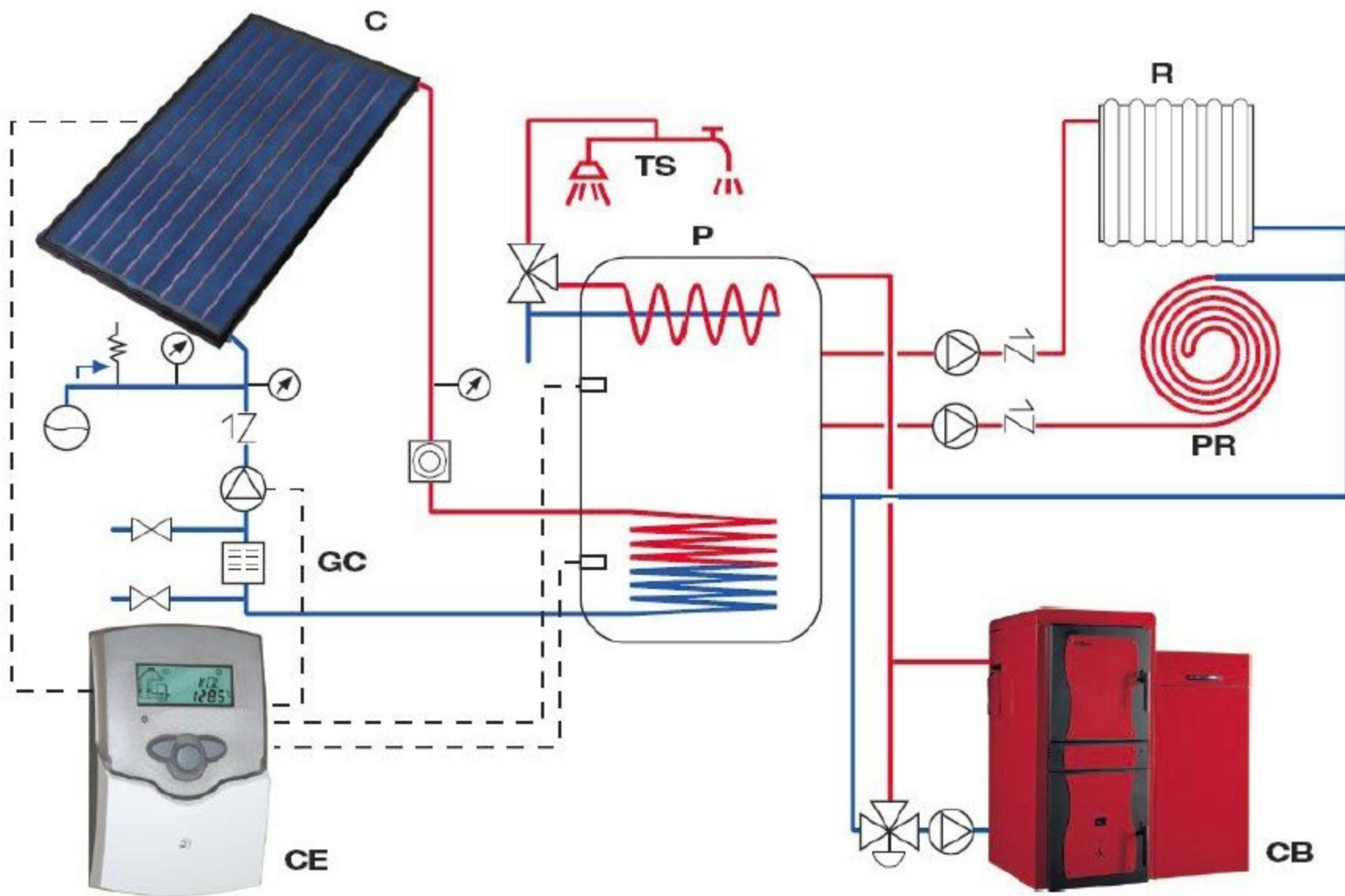
Diagram of solar kit installation for hot sanitary water and supply to the heating with wood or pellet thermo-product.
